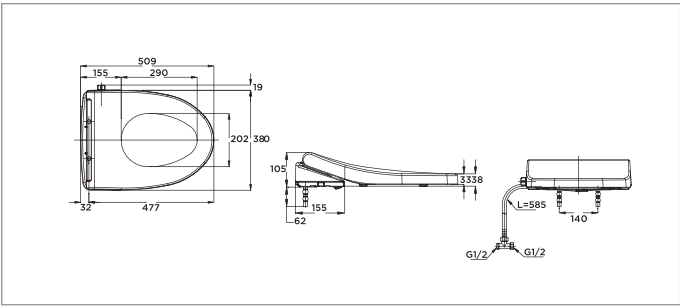
TCW1211A TCW1211A Nắp rửa cơ Ecowasher
